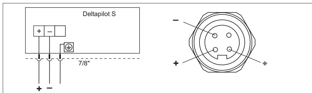
left: Electrical connection for devices with 7/8" plug connector right: View of connector on device
